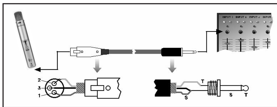
Fig. 3: Using an unbalanced connecting cable.
