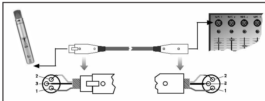
Fig. 2: Using a balanced connecting cable.
