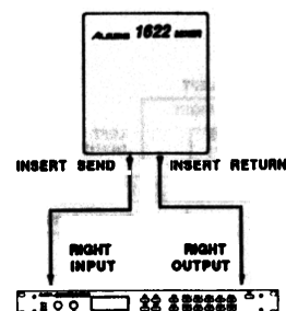
Figure 3 FIGURE 3 CONNECTION TO CONSOLE VIA INSERT PATCH POINTS
