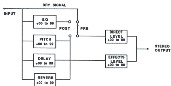
QuadraVerb MIX SECTION Simplified Block Diagram
